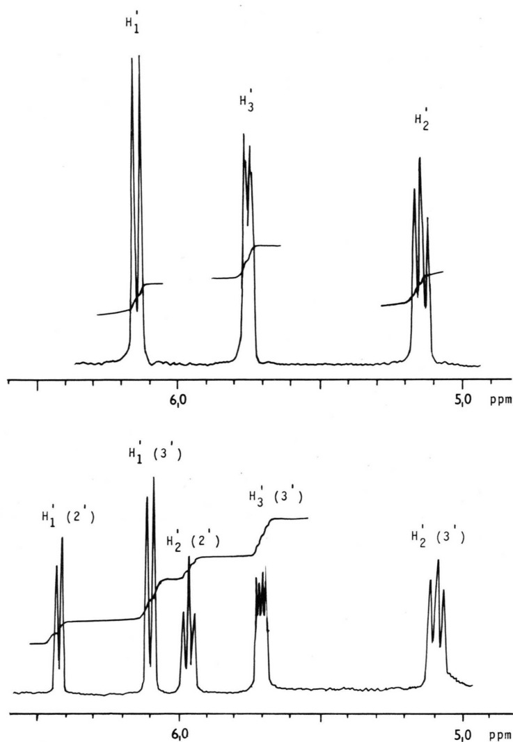
Fig. 1. H 1 ' , H 2 ' , and H 3 ' resonance signals of 3'-O-naphthoyl-1-adenosine (upper spectrum, 50 scans), and naphthoyl-1-ADP ( 10 ) (lower spectrum, 100 scans). 1 H-NMR spectra were taken in DMSO-D 6 /D 2 O (8/1, v/v) at 30 °C with a digital resolution of 0.1 Hz. The concentrations were 10, and 5 mM, respectively. The coupling constant J_{1,2'} of H 1 ' was 5.5 Hz for 2'-, and 7.5 Hz for 3'-isomer (lower spectrum). The isomeric mixture contained 31% 2'- and 69% 3'-ester, as being estimated by integration of H 1 ' resonances.
